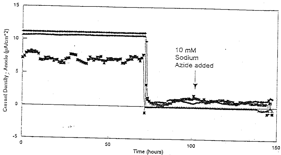
Figure 2. Time plots of measured current flowing between anode and cathode for: (■) & (♦) mixed culture of Desulfovibrio vulgaris and Vibrio sp, (▲) sterile control, with the addition of 10 mM sodium azide at 100 hours, note sodium azide is an inhibitor of aerobic respiration blocking the transfer of electrons from cytochrome a and a1 to O_2 and has no effect on the current being maintained by the mixed culture.
