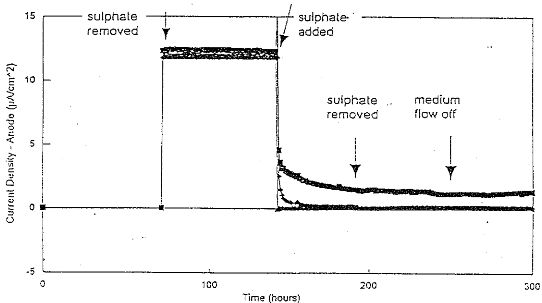
Figure 4 Time plot of measured current flowing between the anode and cathode for (■) and (♦) mixed culture of Desulfovibrio vulgaris and Vibrio sp. (▲) sterile control where sulphate was added for an initial colonisation period of 72 hours while no current was applied, sulphate was then removed while the current was applied and added again when the applied current was removed later sulphate was removed and experiment continued after medium flow was stopped. The current was maintained in one of the mixed cultures even after sulphate was removed and the medium flow was stopped.
