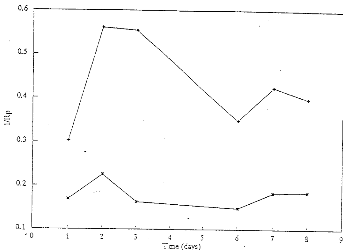
Figure 5. Time plot of the inverse of the polarisation resistance of mild steel coupons exposed to Pseudomonas aeruginosa FRD1 (x) and sterile control (+).
